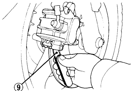
(9) Feeler gauge
