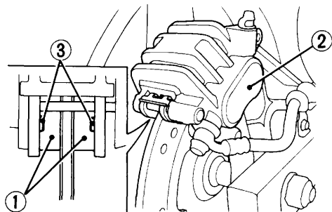
(REAR) (1) Pads (2) Caliper (3) Wear lines
