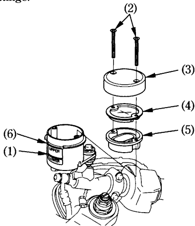
(2) Screws
