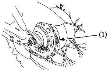
(1) Retaining clip
