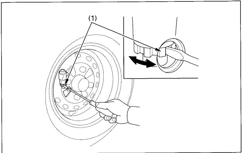
(1) Brake adjusters
