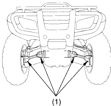
(1) driveshaft boots
