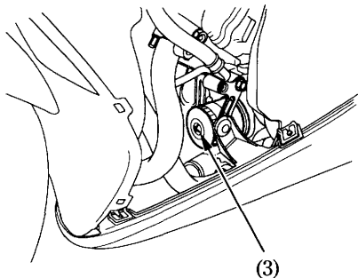
(3) Oil filter
