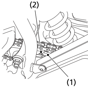
(1) drive chain slider (2) wear limit line
