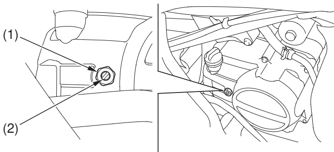
(1) lock nut
