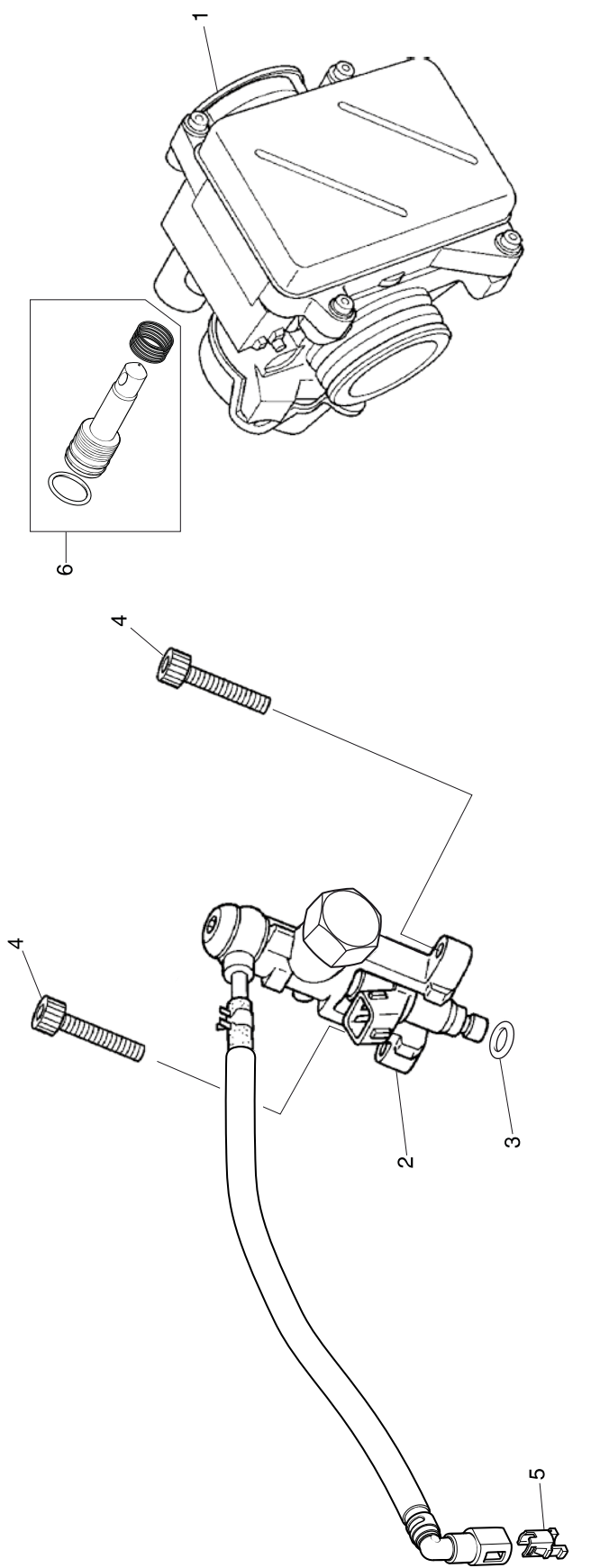
Block No. E-16 Throttle body Injector
